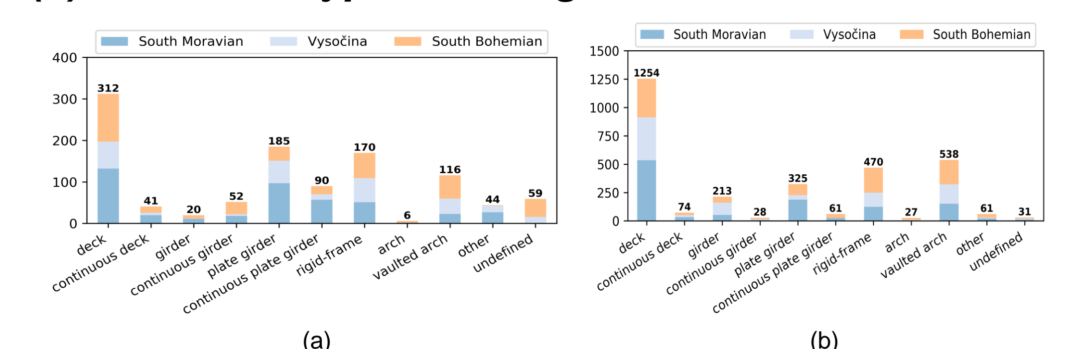
Figure 7: Number of bridges considering the structural type (a) on motorways and 1st class roads, (b) on 2nd and 3rd class roads (ŘSD ČR)
