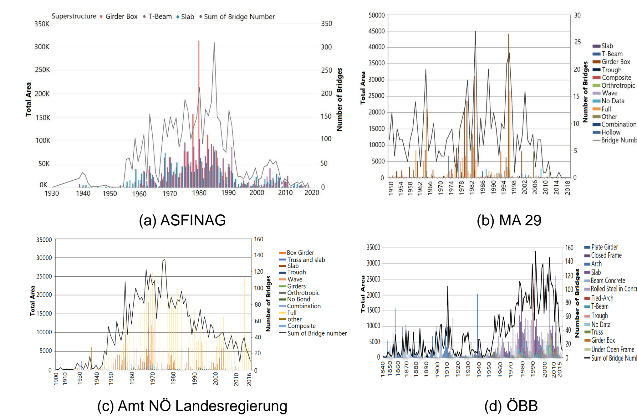
Figure 3: Bridge distribution based on construction year
