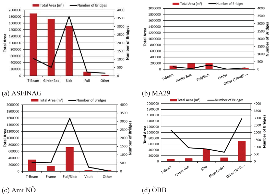
Fig. 1 Bridge distribution in Austria based on the structural type of the cross-section
